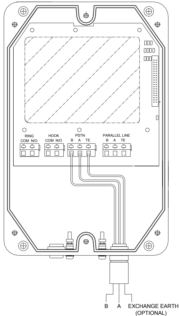
Figure 5- telephone line connections - telephone line only
