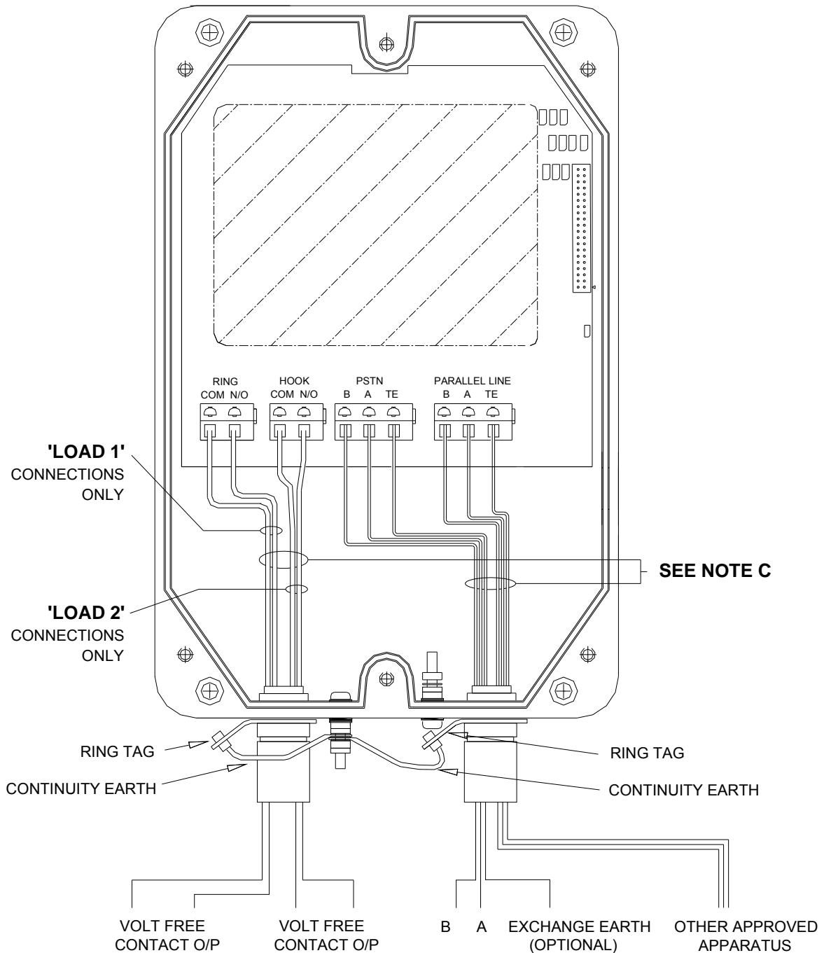
Figure 7 – Wiring for telephone and external loads
