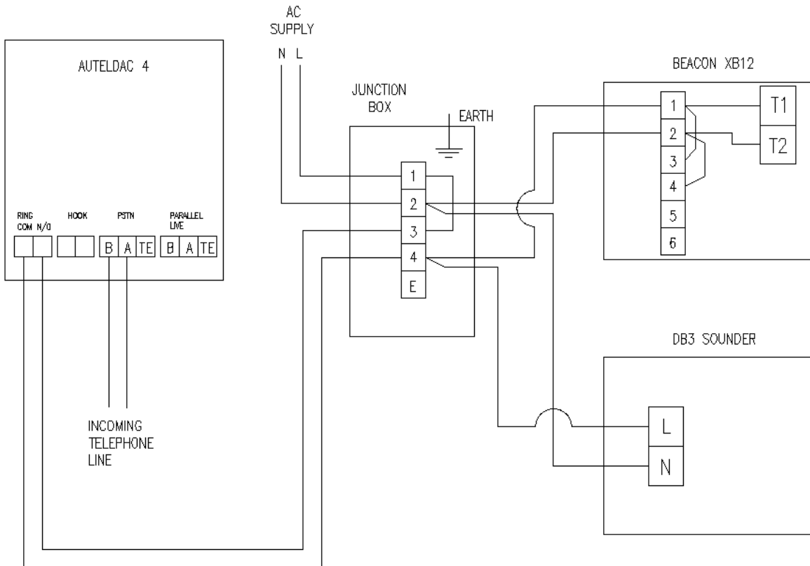
Telephone connection diagram
