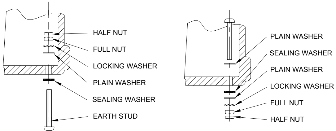
Figure 2 - Internal and external earth bonding stud arrangements
