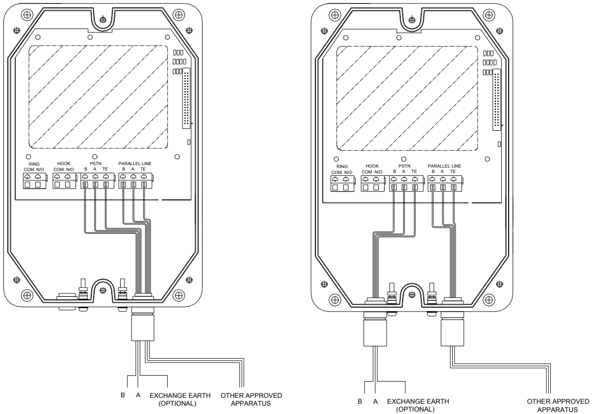
Figure 6- telephone line connection + parallel connection (alternatives)
